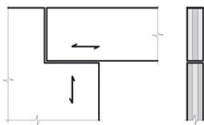
c) Lintel of CLT inserted with horizontal top layer
