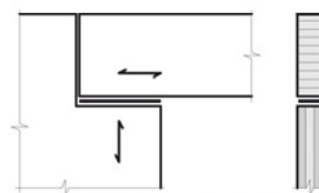
f) ... with inserted steel sheet (support pressure)
