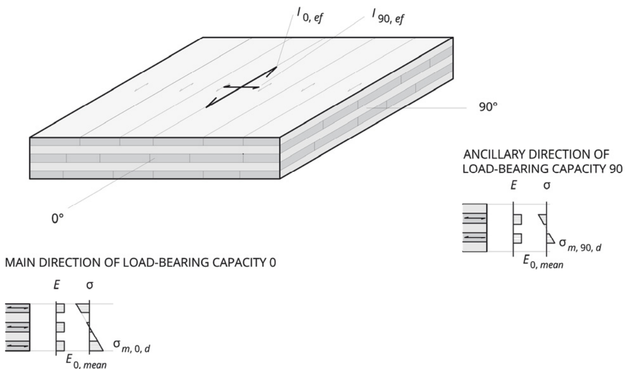
Figure 2-6: Cross-laminated timber element with main and ancillary direction of load-bearing capacity
