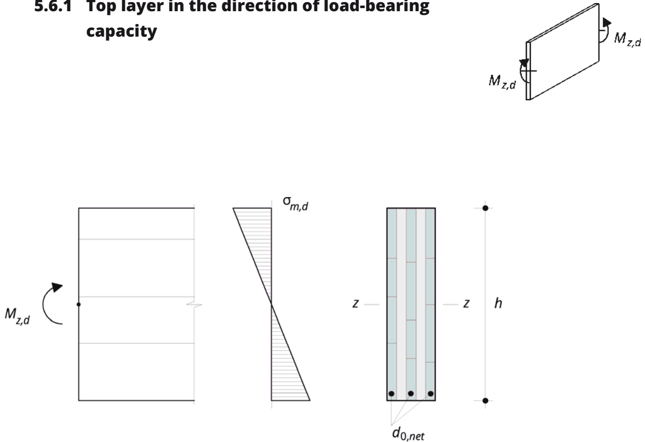
Figure 5-10: Bending stress for girders with a top layer in the direction of load-bearing capacity
