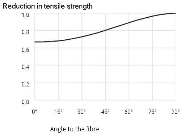
Figure 9-10: Reduction in tensile strength as a function of the angle to the fibre
