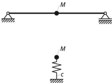
Figure 6-6: Generalised mass
