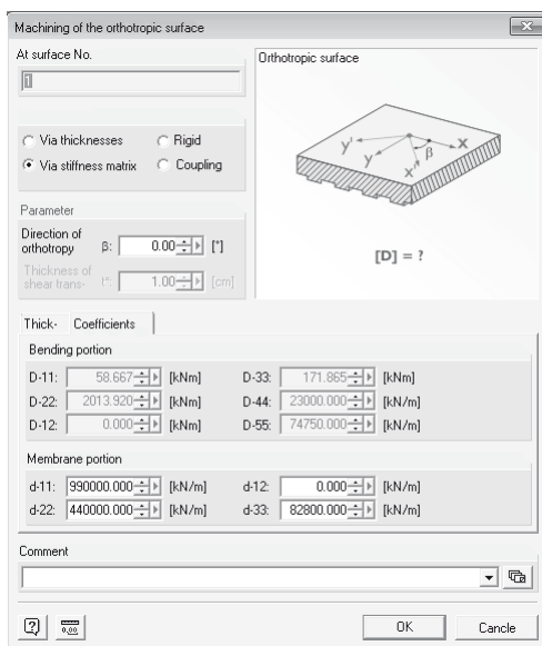
Figure 4-10: Input of the coefficients of the stiffness matrix for plates (software package RFEM, Dlubal GmbH)
