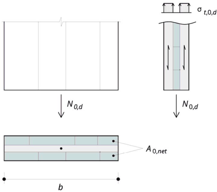
Figure 5-1: Tension in the direction of the top layers
