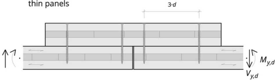
Figure 9-8: Rigid joints
